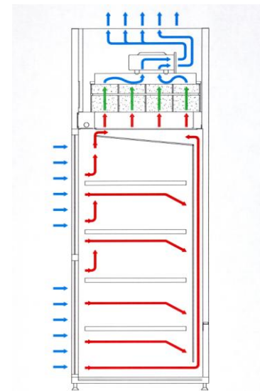
SafeAire™ GS1000-AP Chemical Storage Cupboard
